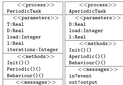
Figure 2: UML task patterns
