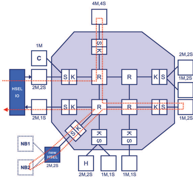
Figure 2. Architecture of companion chip with network on chip.
