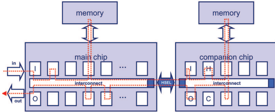
Figure 1. The main TV chip, companion chip, and external memories.
