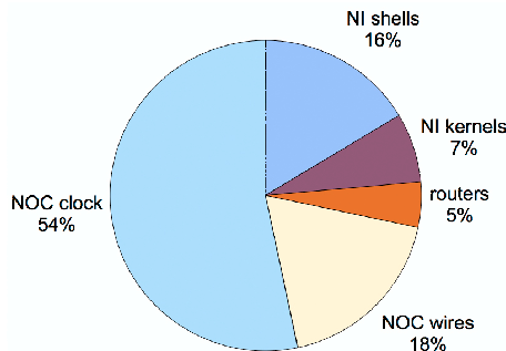
Figure 4. Relative contributions to increase in power dissipation.
