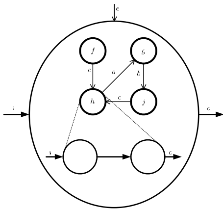
Figure 2: Automaton with process networks
