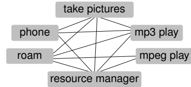
Figure 4. Use-case specification.
