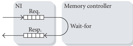
FIGURE 1: Request-response dependency at a memory.
