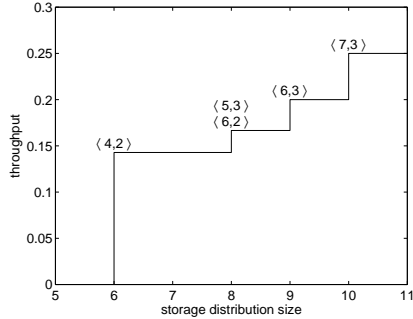
Fig. 2. Pareto space for SDFG shown in Fig. 1.
